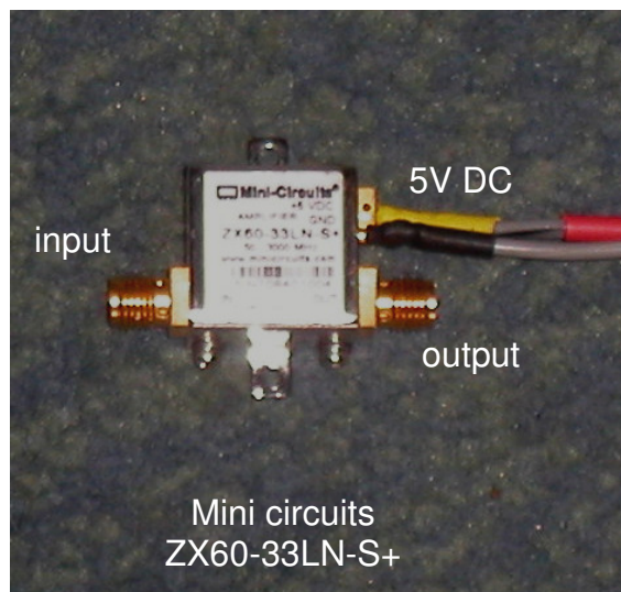
Figure 3.3 ZX60-33LN-S+ device
