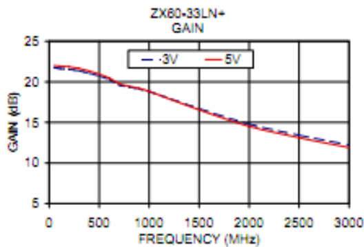
Figure 3.1 ZX60-33LN-S+ Gain
