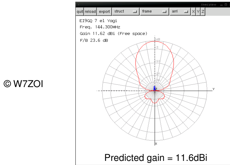
Figure 2.7 Predicted Polar diagram for W7ZOI 7 element Yagi
