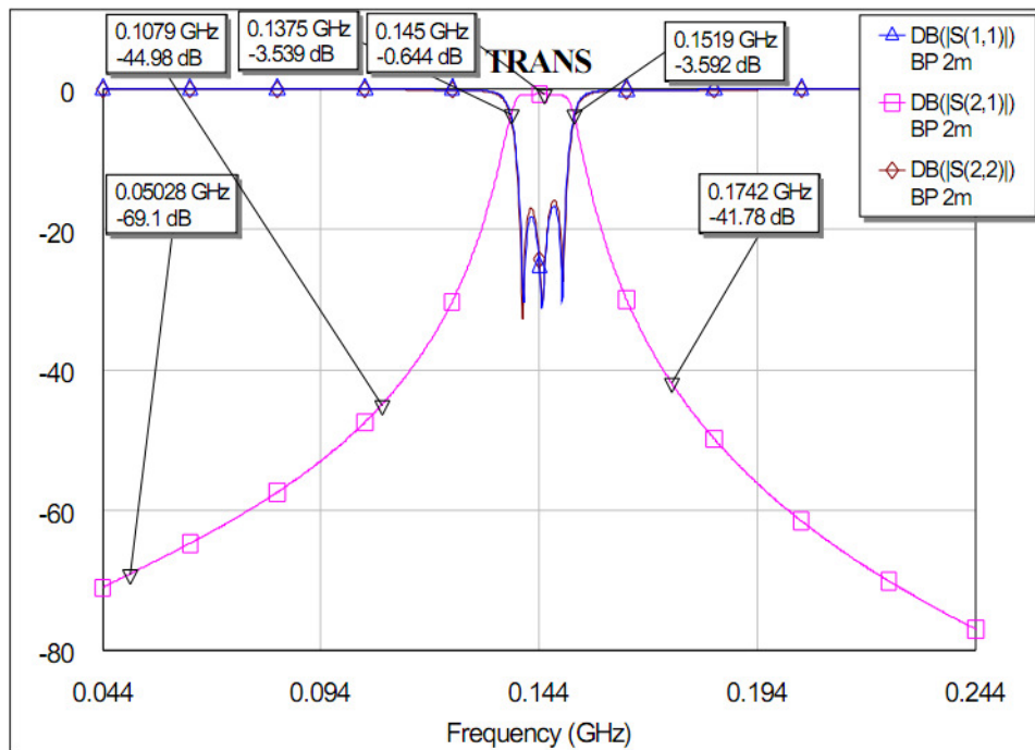
Amplitude frequency response for real C capacitors from Murata and real Q inductors L= self support isolated copper wire diameter 1mm (AVG18) wound at 5 mm 6 turn close wound length 6mm Qo=350 and Frez=901 MHz.
