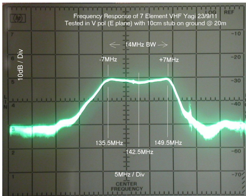
Figure 2.9 Frequency response of 7 Element Yagi
