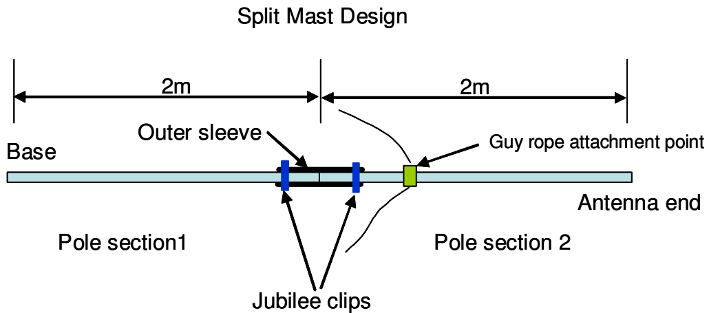
Figure 6.2 Suggestion for a split pole antenna mast
