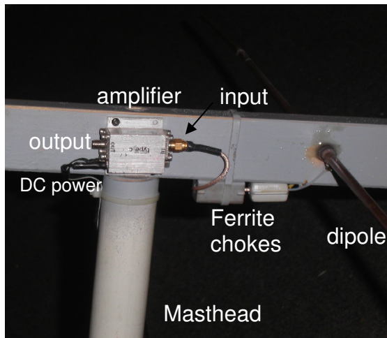
Figure 3.4 Mast head Amplifier
