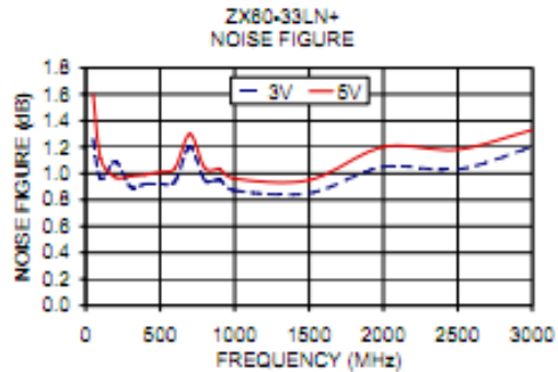
Figure 3.2 ZX60-33LN-S+ Noise figure © Mini circuits
