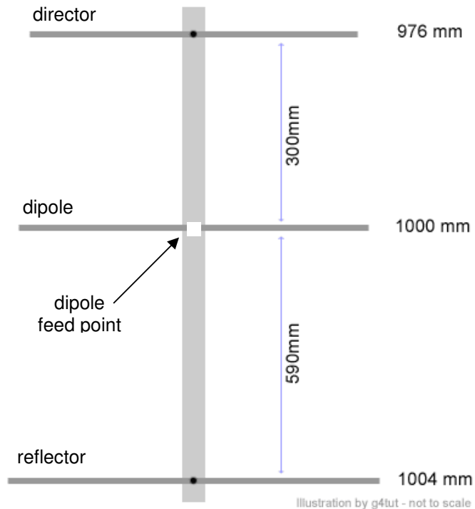
Figure 2.1 A 3 element simple Yagi antenna © Southgate Amateur Radio
