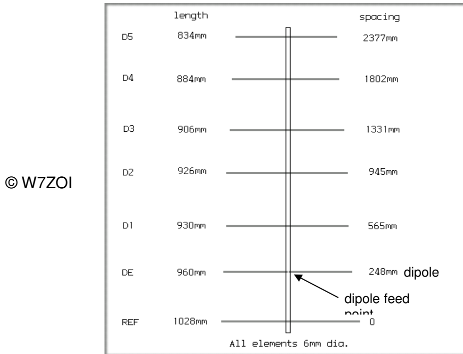
Figure 2.5 W7ZOI 144MHz 7 element Yagi
