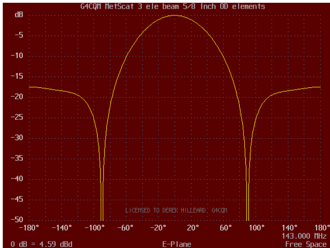
Figure 2.4 Expected -3dB antenna beamwidth © G4CQM
