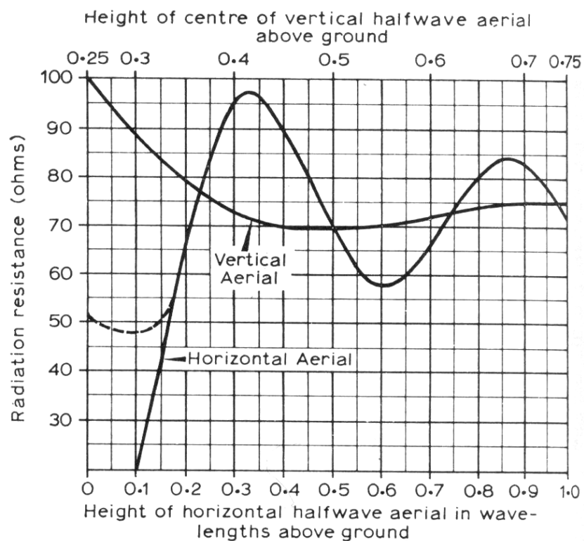
Fig 12.86. Radiation resistance of \lambda/2 horizontal and vertical dipoles as a function of height above a perfect earth.
