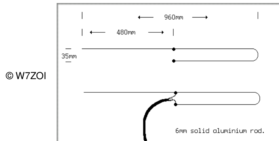
Figure 2.6 Detail and connection to the driven element
