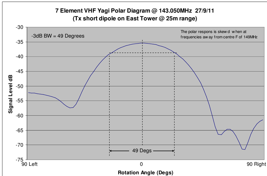
Figure 2.10 7 Element Yagi Antenna Beam Pattern
