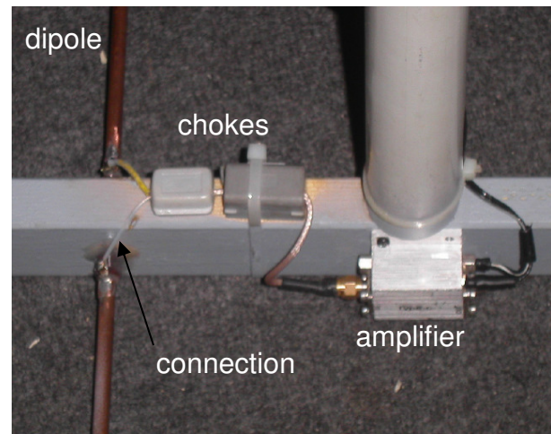
Figure 3.5 Amplifier - RF Chokes & dipole
